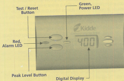
Model KN-COPP-B-LPM with digital display
